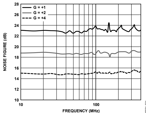
Figure 34. Noise Figure vs. Frequency
